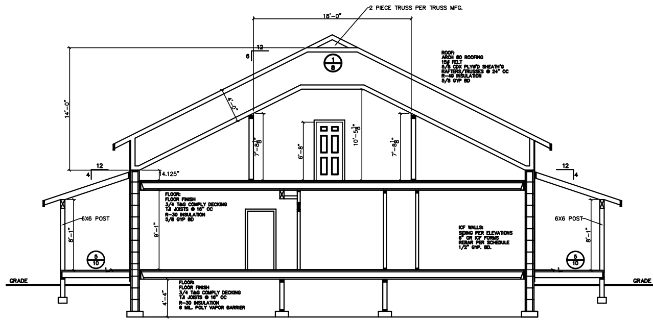
CROSS SECTION CC SCALE: 1/4"=1'-0"
