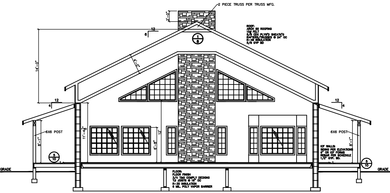
CROSS SECTION BB SCALE: 1/4"=1'-0"
