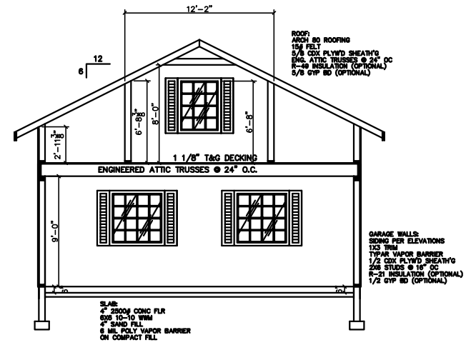
CROSS SECTION AA SCALE: 1/4"=1'-0"
